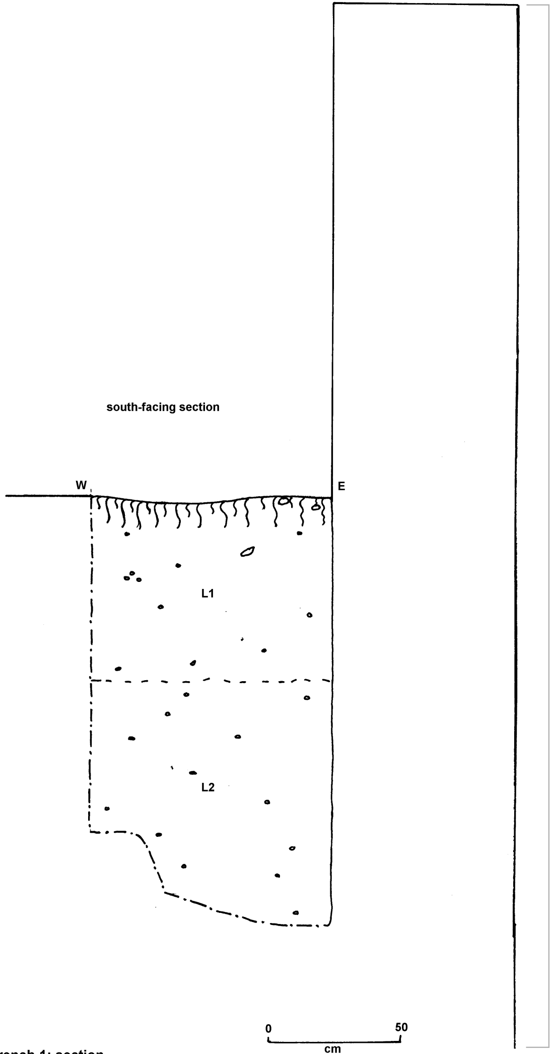
Fig 5 Test-trench 1: section.
